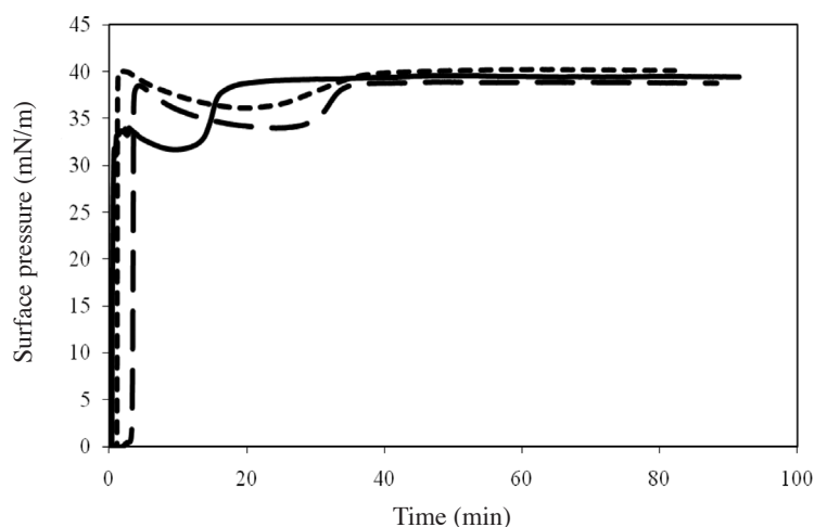
FIGURE 1. Adsorption of surfactin over time at air-water interface
