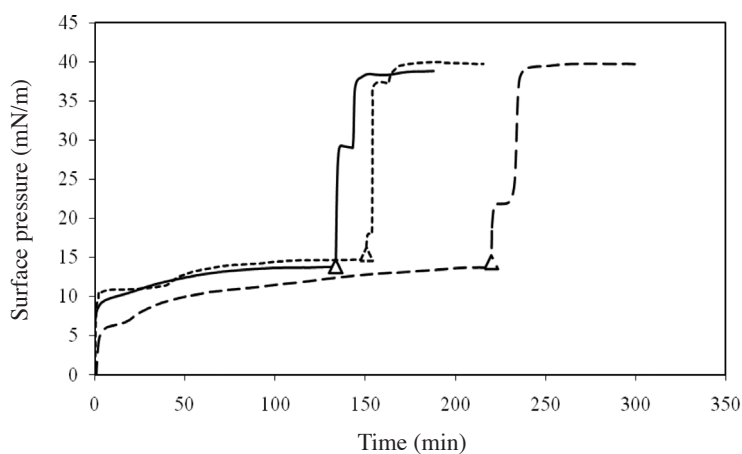
FIGURE 4. Change in surface pressure over time after addition of BSA and subsequent addition of surfactin solution; open filled triangles indicate when surfactin solution was injected
