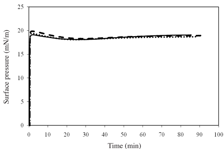
FIGURE 3. Adsorption of \beta -casein over time at air-water interface
