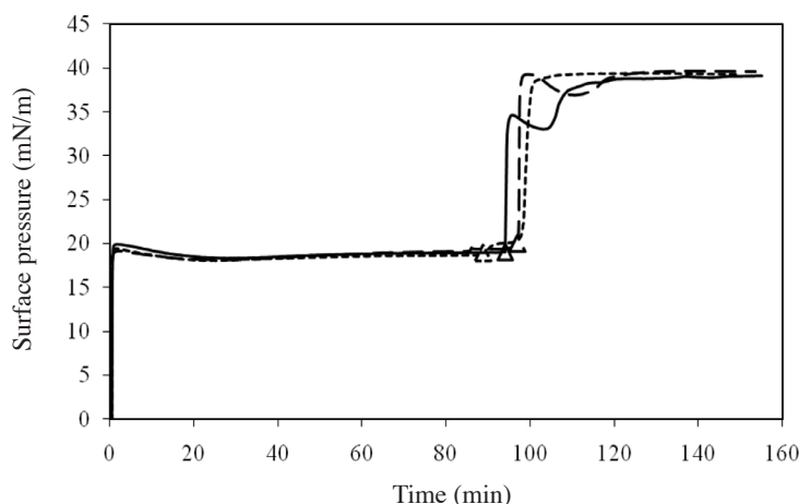
FIGURE 5. Change in surface pressure over time after addition of \beta -casein and subsequent addition of surfactin solution; open filled triangles indicate when surfactin solution was injected
